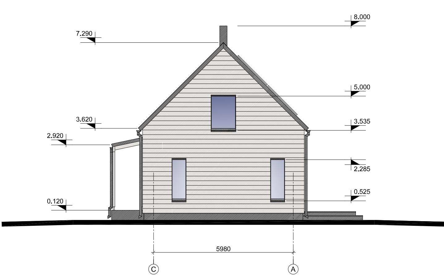
West facade 1:100
