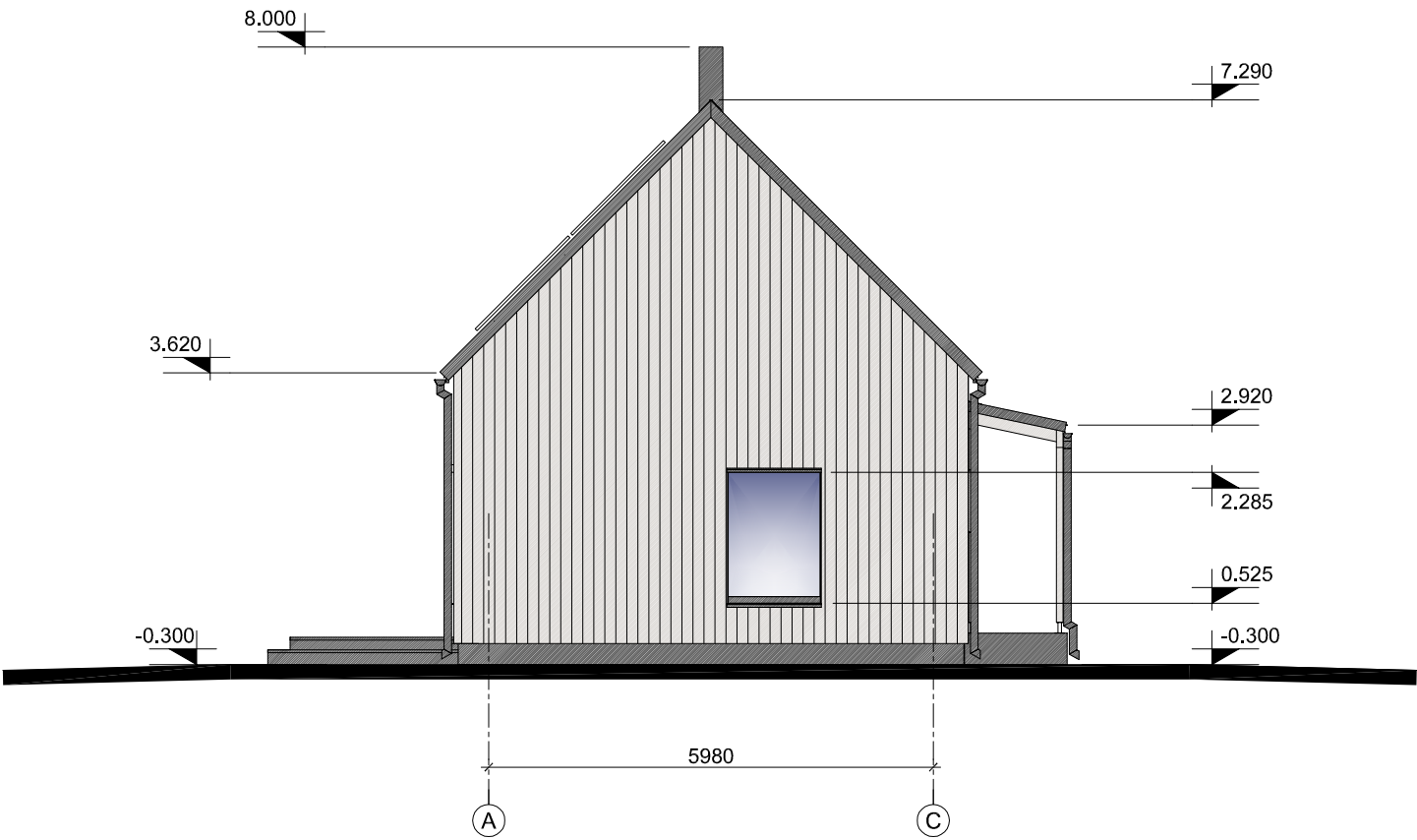
East facade 1:100
