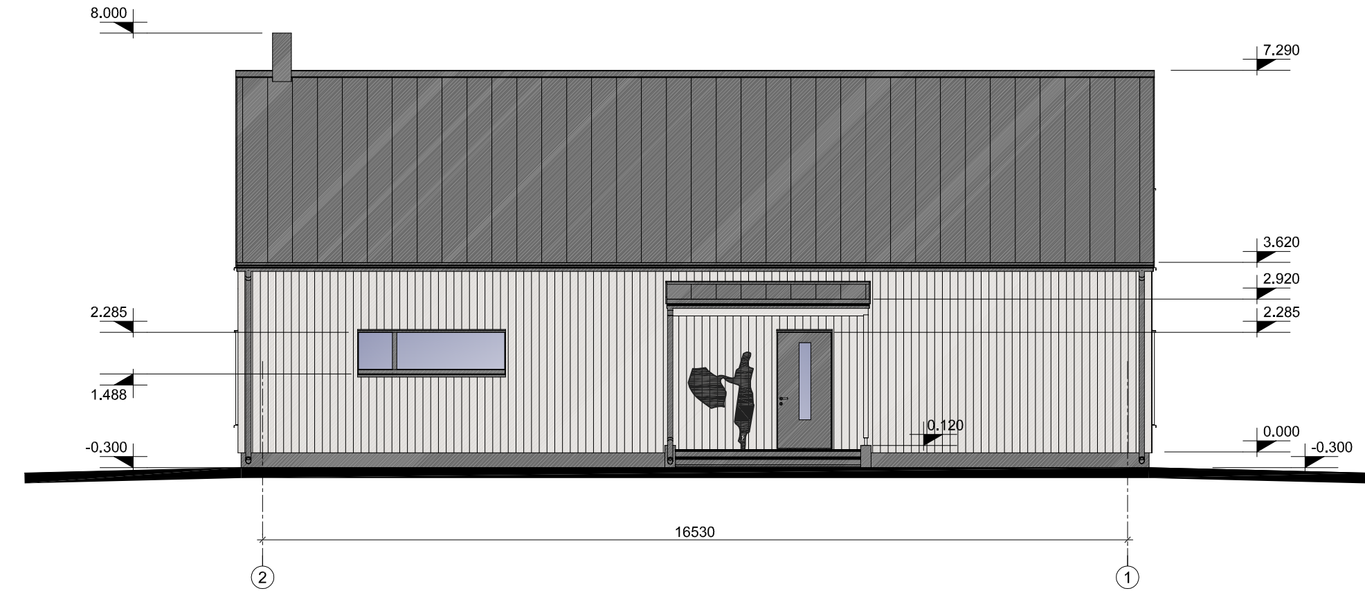
North facade 1:100
