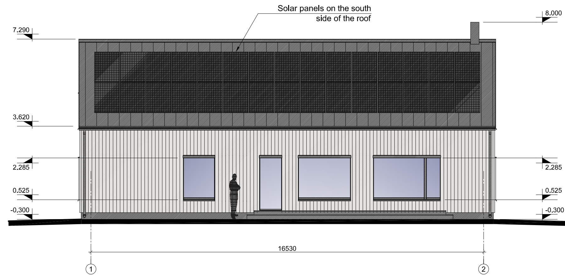
South facade 1:100
