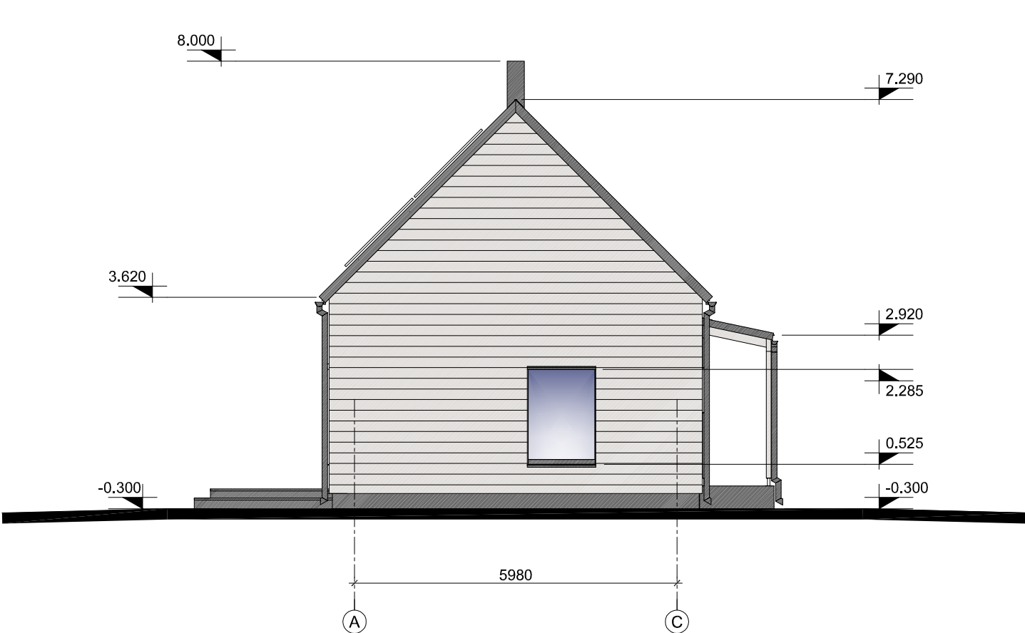
East facade 1:100
